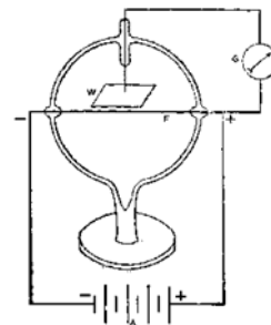
"Diodo" DeForest
